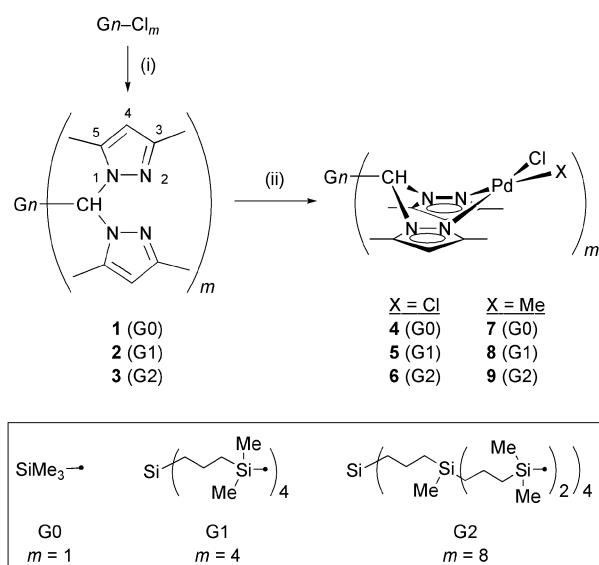
Scheme 2. Synthesis of carbosilane ligands and complexes. Reagents and conditions ( m equiv.): (i) \text{LiCH}(\text{3,5-Me}_2\text{pz})_2 in thf; (ii) [\text{PdCl}_2(\text{cod})] in toluene or [\text{PdClMe}(\text{cod})] in diethyl ether or toluene.
